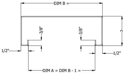
DRYWALL ANCHOR DETAIL
