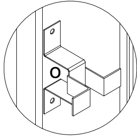
DRYWALL ANCHOR DETAIL
